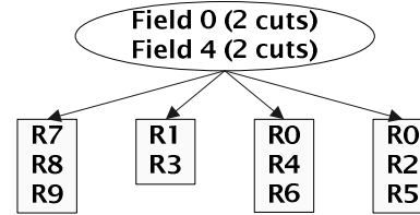
Figure 3: HyperCuts Decision tree (binth 3).
