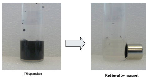
Fig. 2 Magnetic particles ( \text{Fe}_3\text{O}_4 ) easily separated with a permanent magnet. Such magnetic core of the code-carrying particles would allow to retrieve the waste tag on site for decoding and analysis
