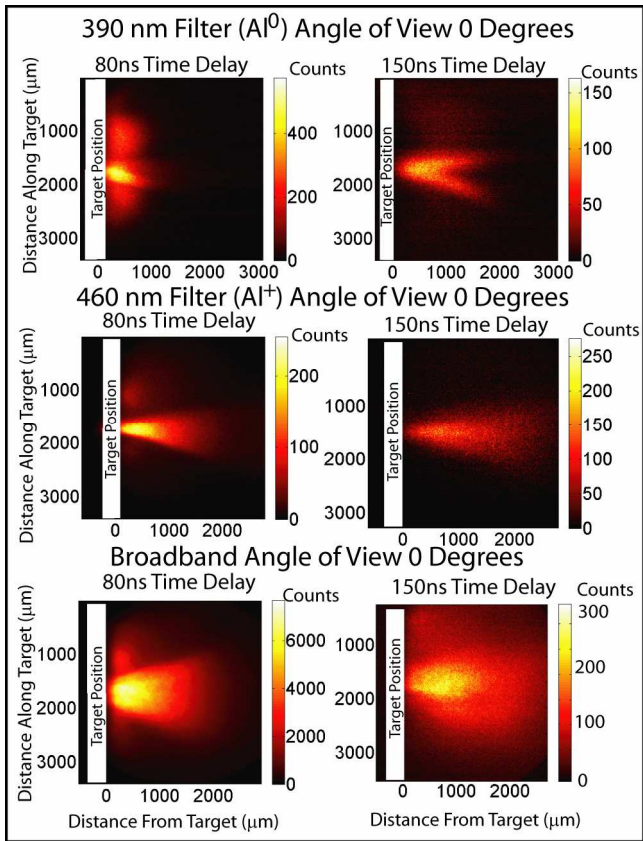
Figure 7: Comparison of emission from Al^0 , Al^+ and broadband imaging for a fixed viewing angle (0 Degrees) for two different delay times (80 ns – left panels and 150 ns – right panels).
