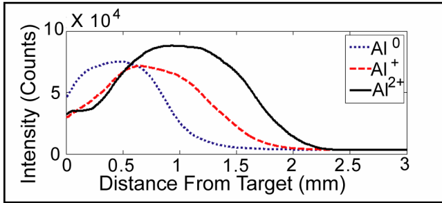
Figure 4: Al 0 (396.15 nm), Al + (358.65 nm) and Al 2+ (360.19 nm) emission as a function of distance from the target at a delay time of 80 ns providing evidence of the space charge effects.
