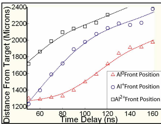
Figure 5: Expansion traces for the luminous front positions of Al 0 (396.15 nm), Al + (358.65 nm) and Al 2+ (360.19 nm) emission emphasising the differences in the spatial evolution of the three ion stages. The smooth curves are best fitted spline curves.
