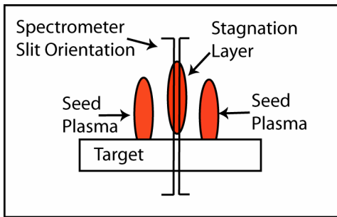
Figure 1: Illustration of the orientation of the spectrometer slit with respect to the stagnation layer. This arrangement provided 1D spatial resolution normal to the target along the stagnation layer.
