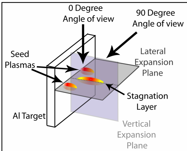
Figure 2: Definition of the viewing angles used for the angularly resolved fast photography with respect to the orientation of the colliding plasmas.
