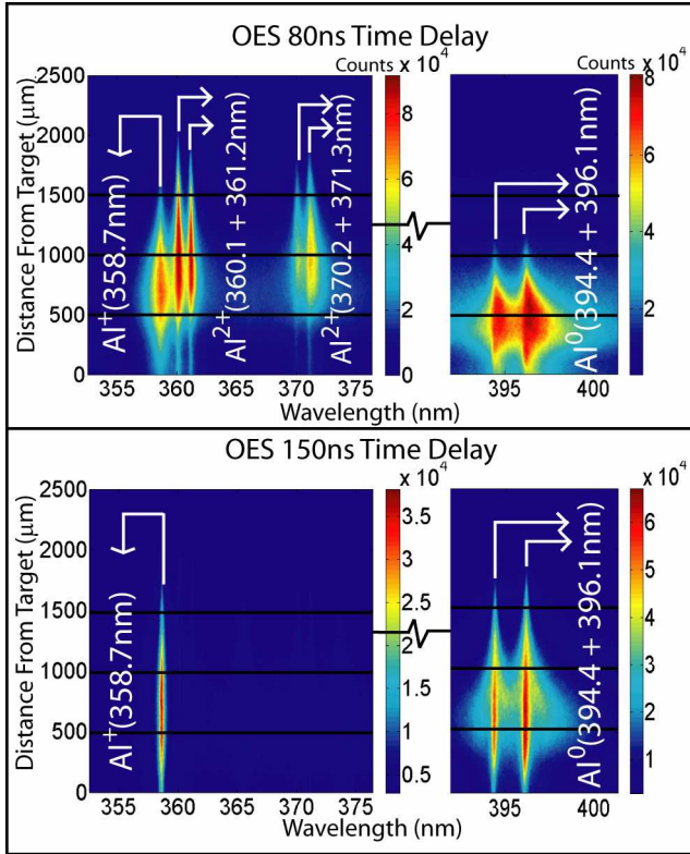
Figure 3: Comparison of the optical spectra obtained showing line emission from neutral, singly and doubly charged aluminium as a function of distance from the target at two different delay times (80 and 150 ns). The black lines serve to highlight the distances of 0.5, 1 and 1.5 mm from the target surface.
