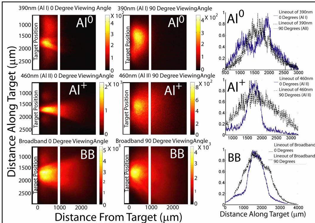
Figure 6: Comparison of the angularly resolved spatial emission from neutral Al atoms with that of singly charged Al ions and broadband emission for the two angles (0 degrees – left panels and 90 degrees – centre panels) defined in figure 2 (recorded at a delay time of 90 ns). The right hand panel shows the comparison of the emission distribution (lineouts) from the two viewing angles along a line parallel to, but separated from, the target surface by a distance of 1 mm. The white lines in the images show where the lineouts were taken for comparison.
