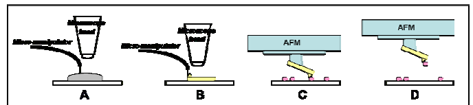
Scheme 1. Microsphere attachment to the AFM cantilever
