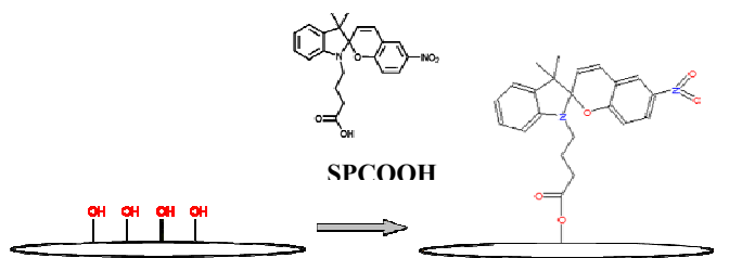
Scheme 2. Immobilisation of SPCOOH to glass slide via DCC coupling chemistry.
