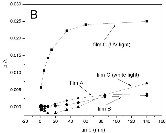
Figure 6. A) Responses of film C upon exposure to UV light and buffer solution of pH=3.5 (dashed line) and deionized water (full line) measured at 431nm (full circles) and 560 nm (open circles). B) Responses of film A (circles), film B (diamonds), film C after exposure to white light (triangles) and UV light (squares) measured at 431 nm.
