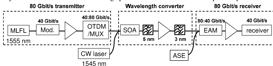
Fig. 1: Experimental setup of wavelength conversion at 80 Gb/s
