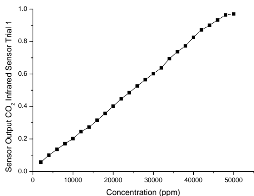
Fig. 1 CO 2 calibration data for IR sensor
