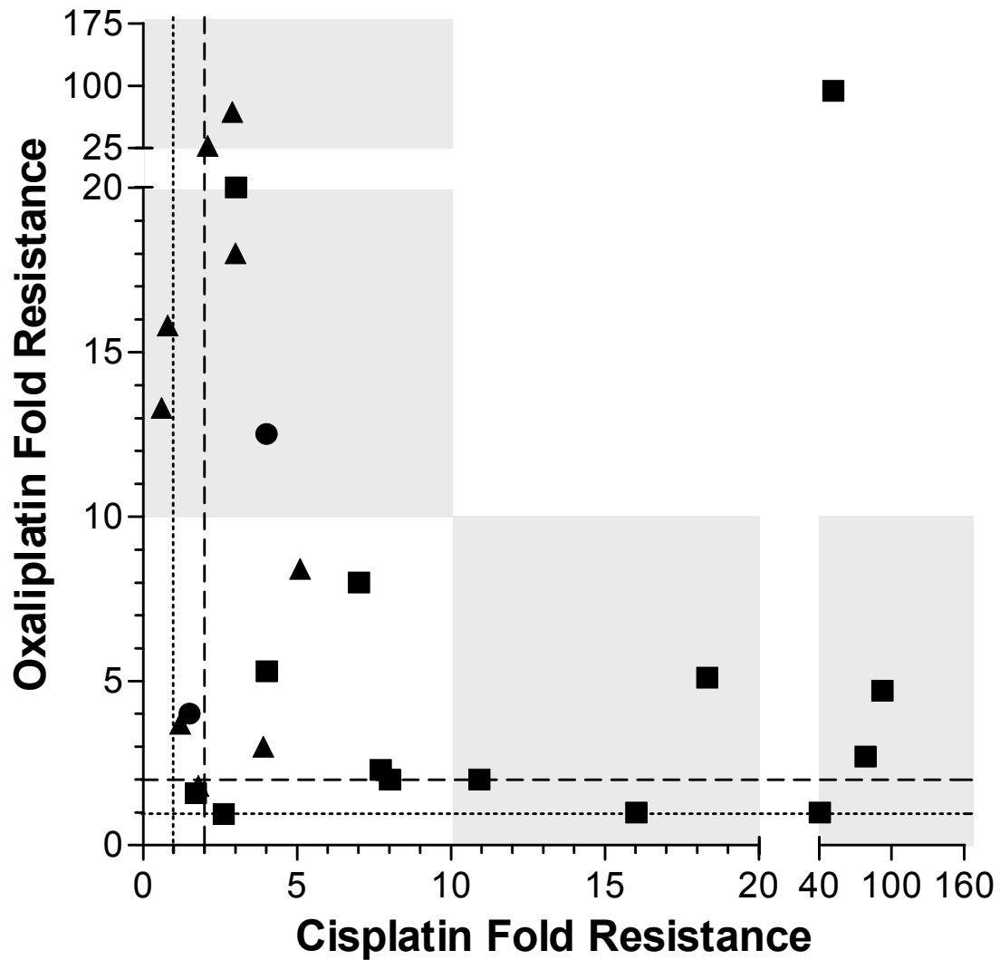
Figure 1 – Cross resistance between cisplatin and oxaliplatin in cell models of acquired platinum resistance. The fold resistance of cisplatin and oxaliplatin of each resistant cell line it was derived from is plotted (from Table 1). Cells developed with cisplatin (■), oxaliplatin (▲) and carboplatin (●) are indicated. The dotted line (...) at 1 indicates the fold resistance of the parental cell lines. The dashed line (---) at 2 indicates the level of clinical platinum resistance.
