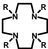
Substituted 1,4,7,10-tetraazacyclodecane
