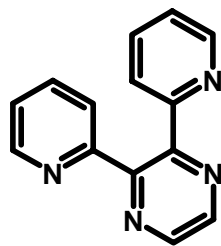
2,3-dipyridopyrazine (dppz)
