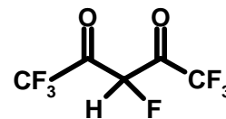
Heptafluoroacetoacetate
