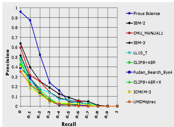
Figure 6: Top 10 manual search runs
