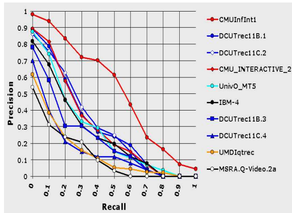
Figure 7: Top 10 interactive search runs
