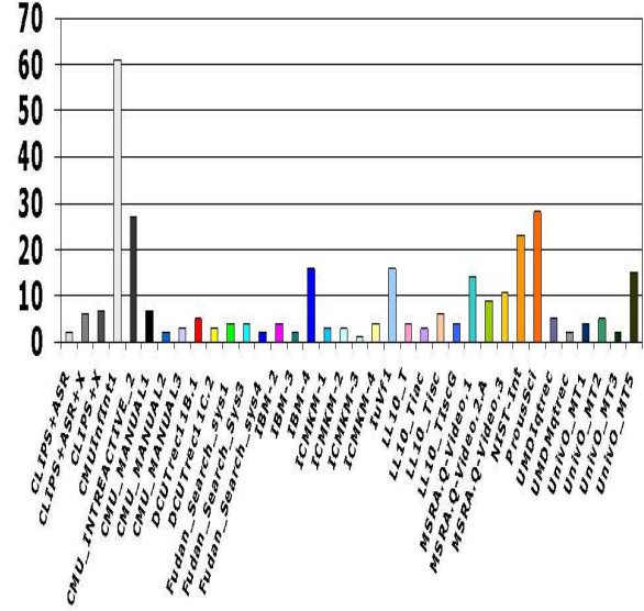
Figure 9: Relevant shots contributed uniquely by run
