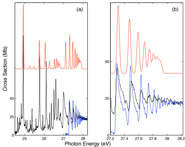
FIG. 2: The experimental absolute photoionization cross section for \text{Rb}^+ in the region of 4p \rightarrow ns, md excitations. (black) DLP, (blue) absolute single-photoionization spectrum and (red) synthetic spectrum shifted by -0.015 eV.
