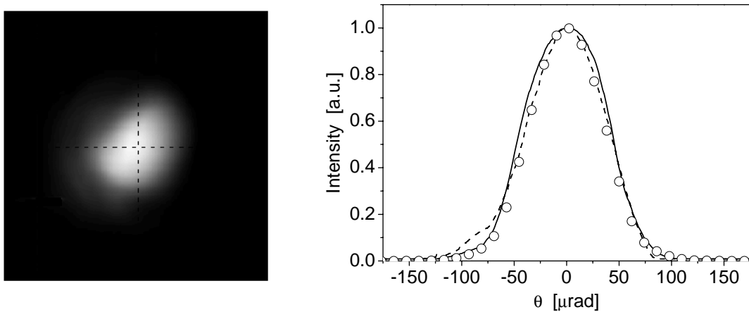
FIG. 3: Spatial profile of the FEL radiation. Left: photon beam image on a Ce:YAG crystal averaged over many shots. The Ce:YAG screen is located 23.5 m downstream of the undulator exit. The FWHM spot size is 2.1 mm. Right: vertical (solid line) and horizontal (dashed line) slices of the image. Circles represent simulation results with the code FAST [38]. The average energy in the radiation pulse was 40 \mu\text{J} . The radiation wavelength was 13.7 nm.
