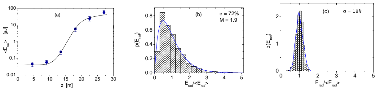
FIG. 4: Energy in the radiation pulse and its fluctuations. Left: Measured average energy in the radiation pulse versus undulator length showing exponential growth and saturation. Error bars correspond to the uncertainty in the calibration of the MCP-detector of \pm 15\% . Center and rightmost panels show the probability distributions for the energy in the radiation pulses. Center plot: end of the regime of exponential growth where the average pulse energy is equal to 1 \mu\text{J} . Rightmost plot: saturation regime where the average pulse energy is equal to 40 \mu\text{J} . Radiation wavelength is 13.7 nm. Solid line on the center plot represents a gamma distribution (4) with the parameter M = 1.9 . The solid line on the right plot represents simulations with the code FAST [38] – see text for details.
