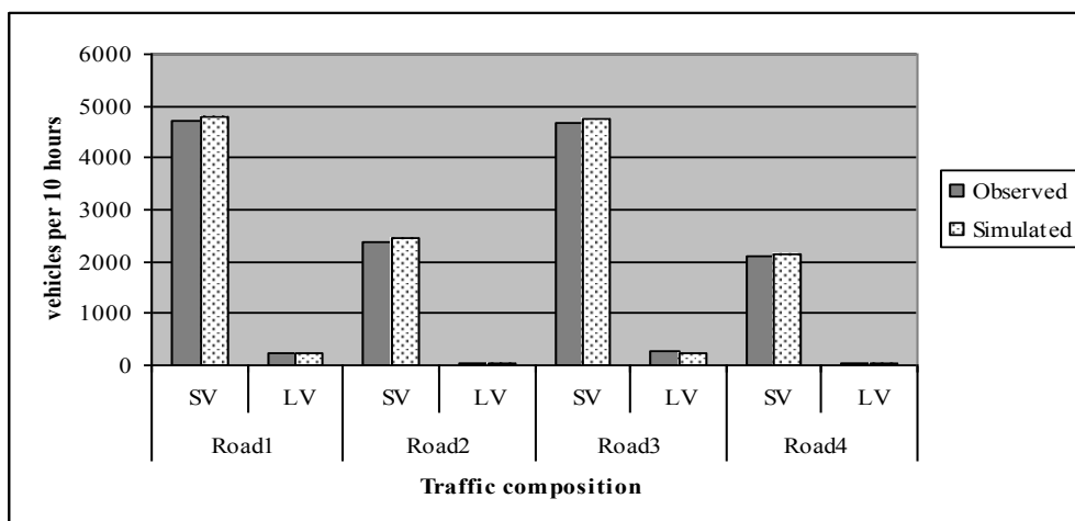
Fig. 5 Model validation (Comparison of Observed and simulated traffic composition data)
