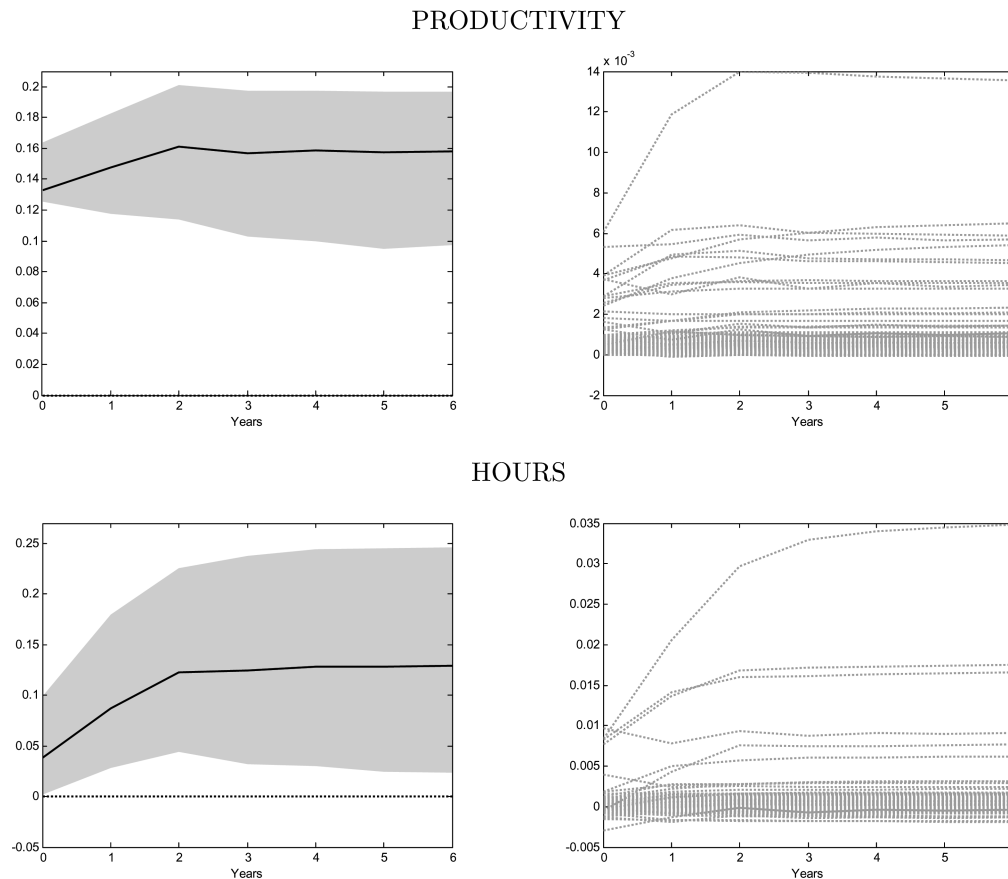
FIGURE 2.—IMPULSE RESPONSES TO TECHNOLOGY SHOCKS WITH SECTORAL INTERACTIONS
