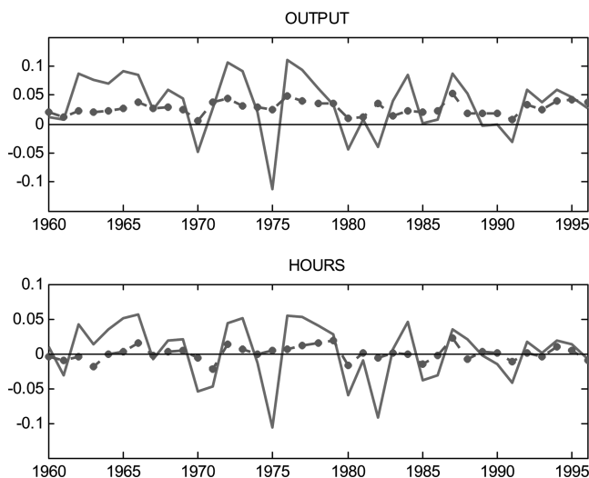
The figure shows the aggregate growth rate of output and hours and the simulated series with aggregate and idiosyncratic shocks but excluding sectoral interactions. The continuous line represents the actual data and the broken line with dots the simulated data with aggregate and idiosyncratic shocks but excluding sectoral interactions.
