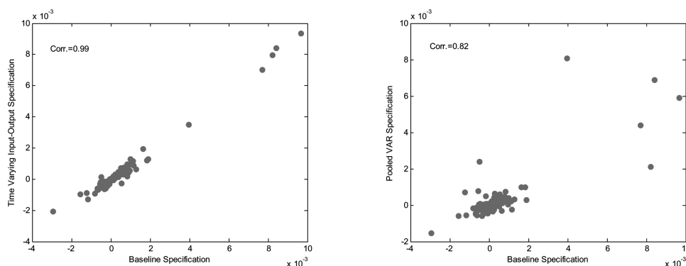
FIGURE 7.—ROBUSTNESS TO VAR SPECIFICATION
