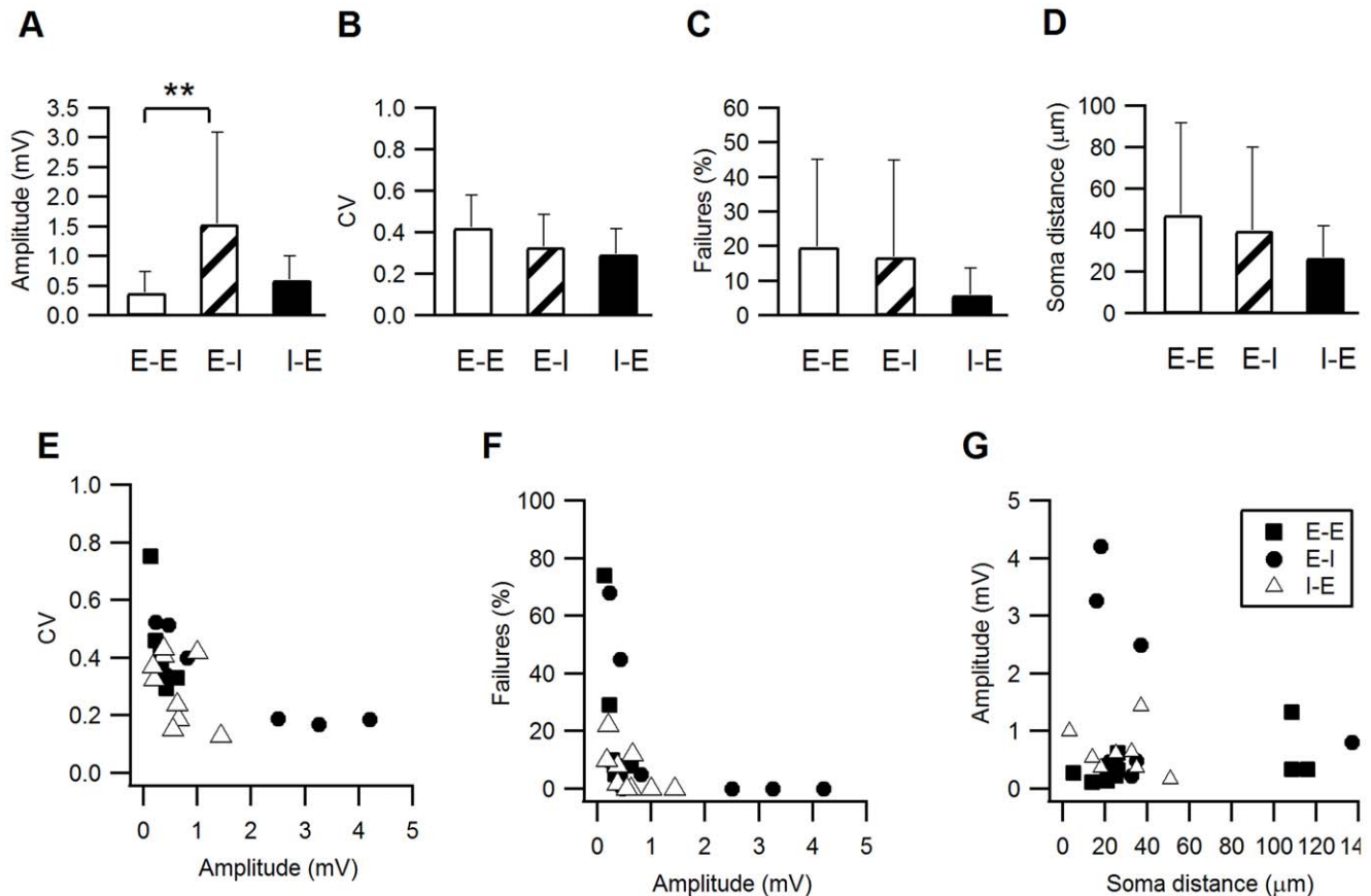
Figure 5. Variance analysis of E-E, E-I and I-E synapses. A–C. The averaged ( \pm s.d.) PSP amplitude (A), CV (B) and percentage failures (C) were compared among the three connection types. The EPSP amplitudes of E-I connections were significantly larger than E-E EPSPs or I-E IPSPs ( p < 0.05 ). I-E connections had on average lower CVs and percentage failures, but these were not statistically significant. D. The average horizontal distances between the pre- and postsynaptic neurons were short for all connection types: E-E 47 \pm 14 , n = 10 ; E-I 40 \pm 14 , n = 8 ; I-E 27 \pm 5 , n = 8 . E–F. The CV and percentage failures of individual synapses were plotted against their average PSP amplitude. In general, larger PSP amplitudes were correlated with lower CVs and percentage failures and smaller PSP amplitudes correlated with the higher CVs and percentage failure. Among medium-sized PSPs no obvious correlations with the CV or percentage failures were observed. G. PSP amplitudes were plotted against the horizontal distance between the pre- and postsynaptic neurons. No correlation could be observed between these parameters (cor. Coeff. = -0.08 ). doi:10.1371/journal.pone.0040601.g005
