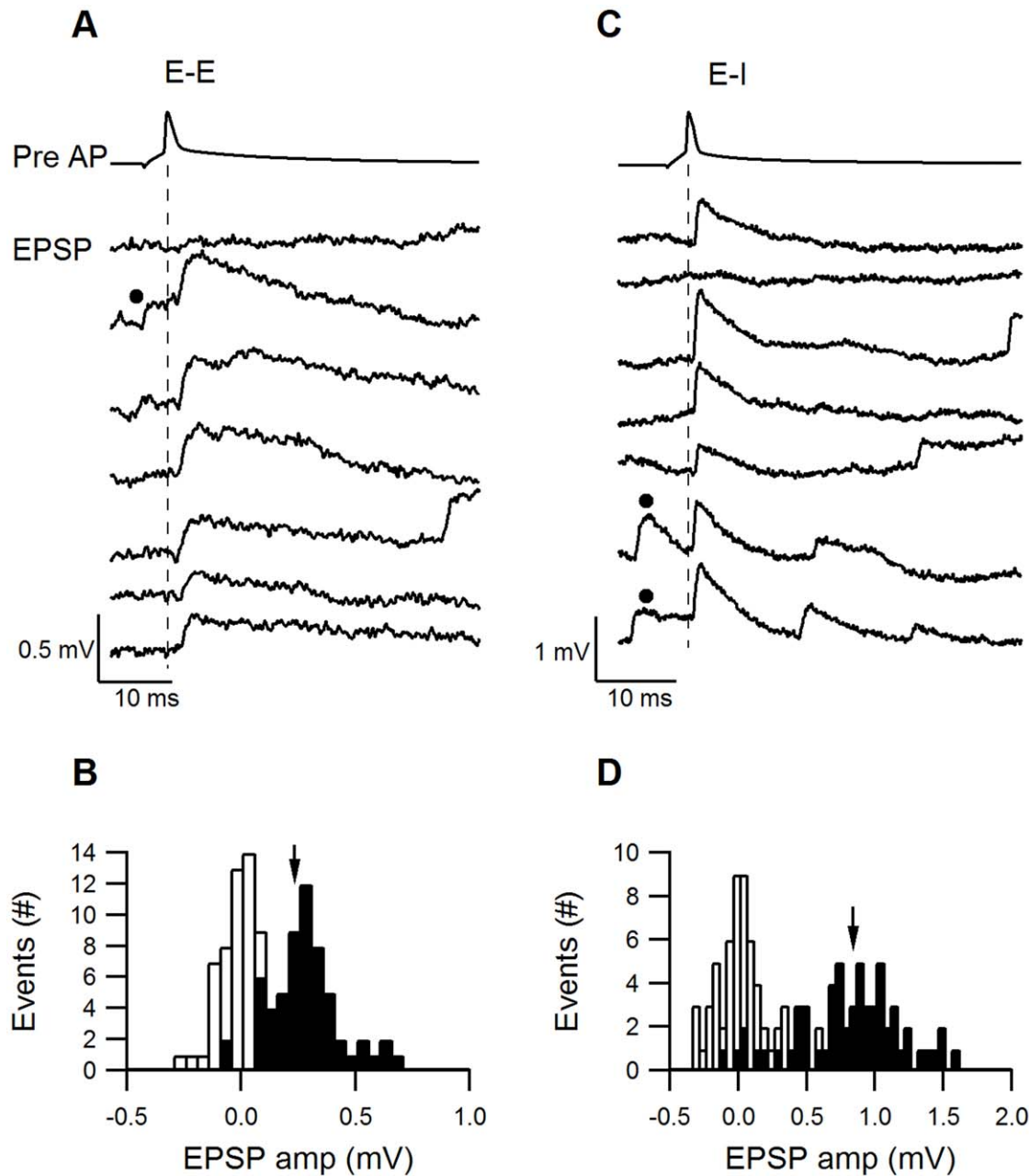
Figure 4. Reliability of E-E and E-I synapses. A. Fluctuations in the EPSP amplitudes at an E-E connection. The upper trace illustrates a presynaptic AP and the 7 subsequent traces show the response evoked in the excitatory postsynaptic cell. B. The EPSP amplitude histogram (filled bars) has a median at 0.24 mV and a \sigma of 0.152 mV. Black dots in A and B indicate spontaneously occurring EPSPs prior to stimulation. C. Fluctuations in the EPSP amplitudes at an example E-I connection. The upper trace illustrates a presynaptic AP and the 7 subsequent traces show the response evoked in the inhibitory postsynaptic cell. D. A broad distribution of the E-I EPSPs, with a median at 0.84 mV and a \sigma of 0.435 mV. doi:10.1371/journal.pone.0040601.g004
