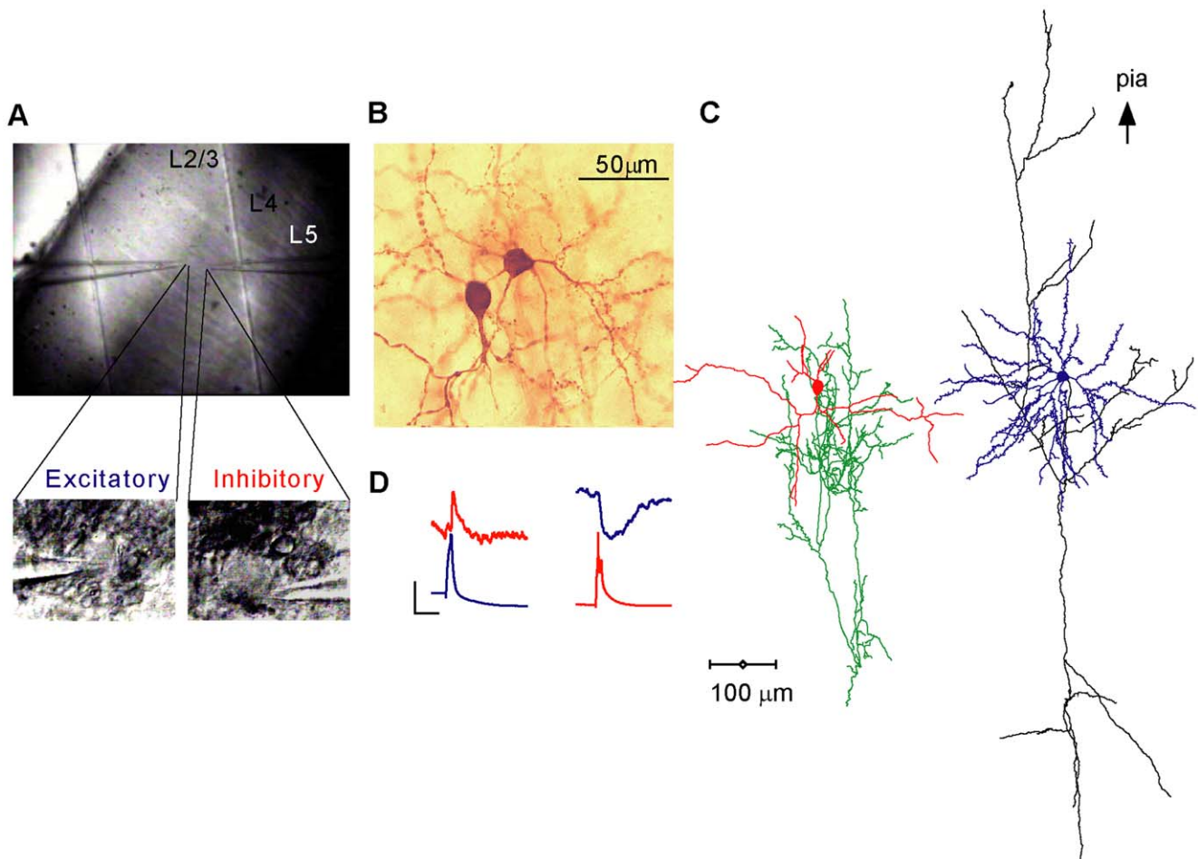
Figure 1. Paired recordings from visually identified L4 neurons. A. An IR-DIC image of a coronal slice from area 17 of the cat cortex. Layer 4 was identified under low magnification (10 \times ) as a dark stripe extending over the middle third portion of the cortex. Lower panel: at a higher magnification (60 \times ) an excitatory neuron (left) and an inhibitory neuron (right) were recorded simultaneously with patch clamp pipettes. B, C. Biocytin stain of the same cell pair and its 3-D reconstruction, identifying them as a spiny stellate cell and a smooth basket cell. The cells are presented separately for clarity. D. The cell pair was reciprocally connected as is evident by the EPSP (red) and IPSP (blue) evoked in the basket and spiny stellate neurons, respectively. The presynaptic APs in the basket and stellate cells are colored blue and red respectively. Vertical scale bar is 0.4 mV for the EPSP/IPSP and 50 mV for the APs and horizontal scale bar is 20 ms. doi:10.1371/journal.pone.0040601.g001
