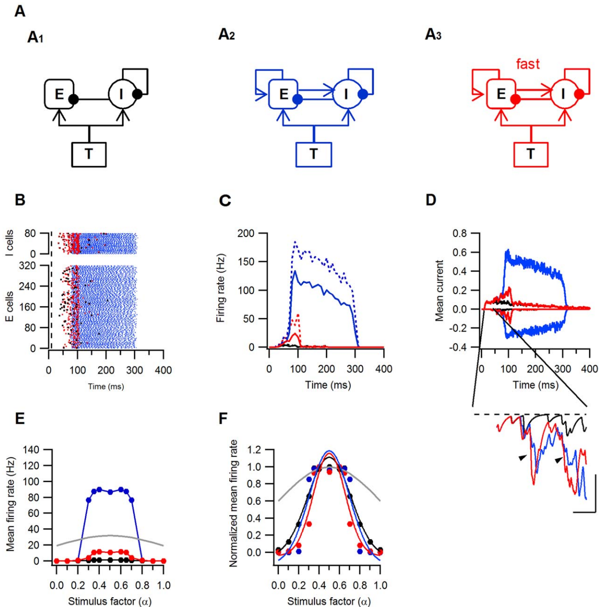
Figure 9. Effects of fast E-I recruitment on the activity and tuning curves of a model recurrent L4 network. Three models were used to simulate activity in the recurrent network. All models included excitatory (E) and inhibitory (I) L4 neurons and feedforward thalamic (T) input synapses and were identical in all but the recurrent excitatory synapses. Excitatory and inhibitory synapses were drawn with arrows and filled circles, respectively. A1. The feedforward model in which E-E and E-I synapses were silenced. A2. The second model incorporating recurrent E-E and E-I synapses with identical kinetics and latencies. A3. The third model is structurally identical to A2 but E-I synapses have faster kinetics and shorter latencies. Models 1, 2 and 3 and all the results are colored black, blue and red, respectively. A-D. Responses of all three models to the same feedforward synaptic input ( F_{in} = 29.5 Hz). B. Raster plots of the excitatory (E) and inhibitory (I) spike times, dashed line marks stimulus start. C. Peri-stimulus histogram of the firing rates of the excitatory (solid lines) and inhibitory (dashed lines) neurons binned at 10 ms intervals. D. Mean excitatory (positive to 0) and inhibitory (negative to 0) currents to the excitatory L4 neurons. Current is given in arbitrary units. The inset shows the mean inhibitory current between t = 40 and 80 ms from simulation start. The arrowheads point towards the earlier onset and faster rise of the current in model 3 compared to model 2. Scale bars are 10 ms and 0.03 I. E-F. Tuning curves of the excitatory neurons. E. Mean firing rates as a function of the stimulus parameter \alpha , note the many-folds amplification of the responses in models 2 (blue) and 3 (red) in respect to model 1 (black). F. The mean firing rates normalized to the maximal response as a function of \alpha . The lines represent the best Gaussian fits to the normalized responses. The grey line is the normalized input frequency. Note the narrowing of the tuning curve in model 3. doi:10.1371/journal.pone.0040601.g009
