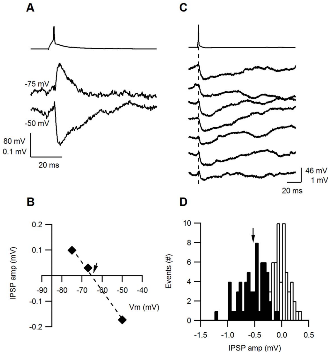
Figure 3. Inhibitory synapses. A. An AP evoked in the presynaptic inhibitory neuron and the simultaneously recorded IPSP (average of 15 traces, each) from the postsynaptic excitatory neuron at two membrane potentials. The IPSP was hyperpolarizing at a V_m of -50 mV but depolarizing at -75 mV. B. The IPSP amplitude plotted as function of the membrane potential ( V_m ). The data were fitted with a straight line (dashed) intercepting the x-axis (indicated by an arrow) at -65 mV. C. In 7 subsequent traces, IPSP amplitudes varied in response to single presynaptic APs, but no failures were observed. The postsynaptic V_m was held at -50 mV. D. A histogram of the IPSP amplitudes (filled bars) was constructed from 60 traces and the background noise (empty bars). The IPSP histogram was fitted with a Gaussian distribution with a median at -0.53 mV (arrow) and a \sigma of 0.36 mV. doi:10.1371/journal.pone.0040601.g003
