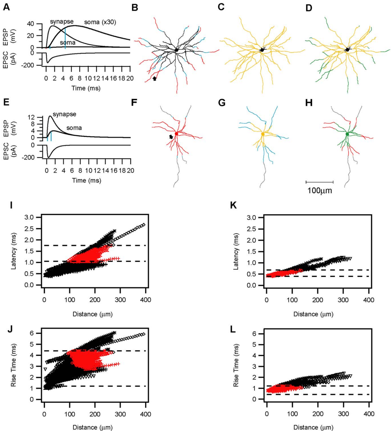
Figure 7. Compartmental model simulations of synaptic kinetics. Electrotonic attenuation of the synaptic current along the dendrites en route to the soma, results in smaller and slower somatic EPSPs. A, E. A single synaptic contact with a conductance of 3.8 nS was simulated on (A) a spiny stellate or (E) a basket cell dendrite at the location where a putative contact was identified (arrows in B and F , respectively). The decay time constant ( \tau_2 ) of the conductance in E was faster than in A (1 ms vs. 2.3 ms). The simulated EPSCs and the resulting EPSPs at the synapse are drawn in a thin line. The same EPSPs measured in the soma are drawn with a thick line. In (A) the somatic potential trace was multiplied ( \times 30 ) to allow direct comparison of the kinetics. The 10% and 90% EPSP amplitudes are marked by the blue lines. Note that the more distal contact simulated in A is more strongly delayed, slowed and attenuated than the proximal contact simulated in E . B–H. A single synaptic activation was simulated successively in all compartments of the spiny stellate ( B–E ) and smooth basket ( F–H ) neurons. In each compartment, the latency of the EPSP arrival at the soma and the somatic 10%–90% EPSP rise times were analyzed and compared with the experimentally observed values. The somatic and dendritic compartments were then colored according to the following categories: Black: simulated values lower than the smallest experimentally observed latency or rise time. Grey: simulated values larger than the largest experimentally observed latency or rise time. Blue: simulated values within the range between the smallest and the largest observed values. Red: Mean EPSP latency (average \pm s.d.). Yellow: Mean EPSP rise time (average \pm s.d.).
