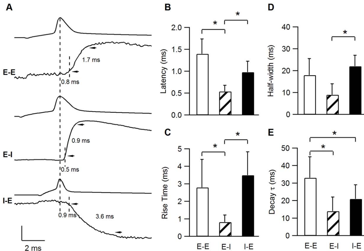
Figure 6. Synaptic Kinetics. A. Averaged PSPs from 3 individual connections illustrate the differences in synaptic kinetics of the various connection types. The presynaptic APs were aligned at their peak (depicted by the long dashed line). The short dashed lines on every PSP denote the time at which the PSP rose to 10%. The latency between the presynaptic AP peak and the 10% PSP was 0.8, 0.5 and 0.9 ms for the E-E, E-I and I-E synapses, respectively. The arrowheads point towards the 10% and 90% values of the PSP amplitude and the delay between them is defined as the rise time. Vertical scale bar represents potential and was 80 mV for all three APs and 0.13 mV, 0.85 mV and 0.2 mV in the E-E, E-I and I-E PSPs, respectively. B-E. E-I connections have significantly shorter latencies and faster rise times compared with E-E and I-E connections. All bar graphs represent the averaged values \pm s.d.
