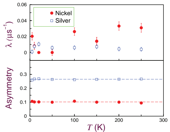
FIG. 3. The temperature dependence of the damping rate (top) and asymmetry (bottom) at 14 keV in nickel (red circles) and silver (blue squares), measured in zero field.
