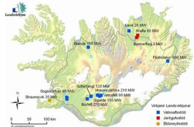
Hydro power plants in Iceland
