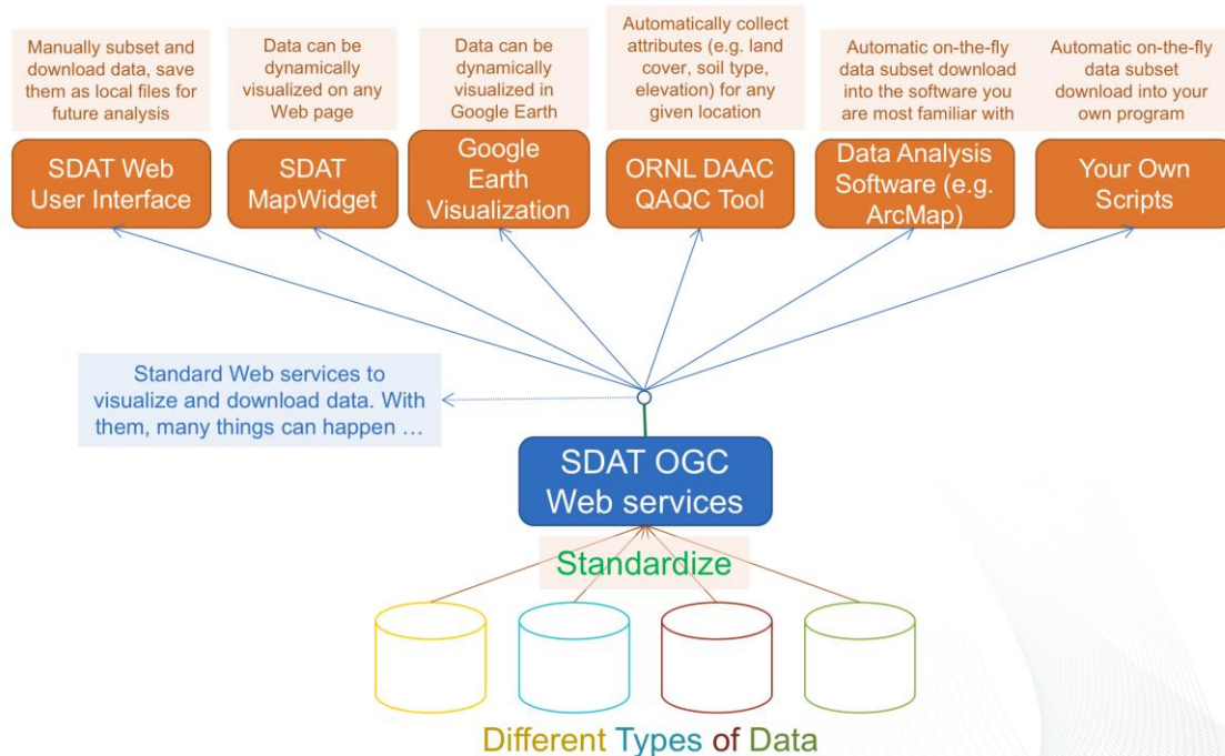
Figure 1. Spatial Data Access Tool (SDAT) framework
