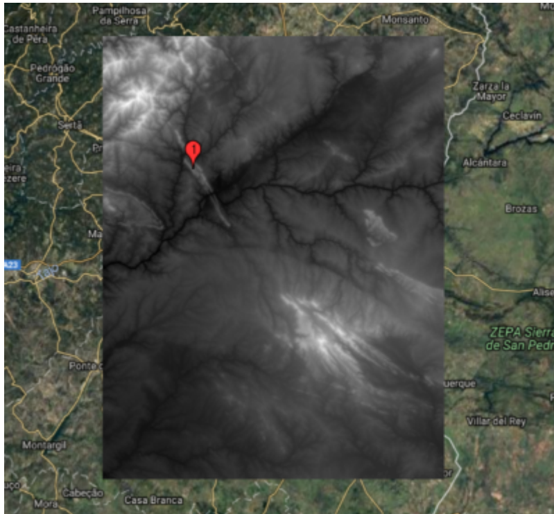
Figure 3.2: 1 arc-second (~30 meter) resolution SRTM elevation map of the Perdigão site. The GeoTIFF file (and other formats) can be downloaded from earthexplorer.usgs.gov
