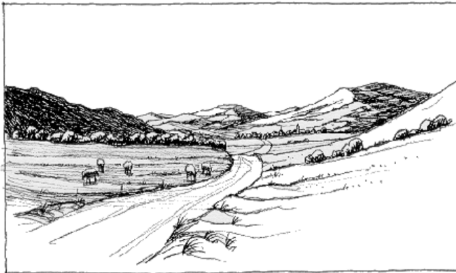
Figure 3.1: Illustration of orography (elevation) from the European Wind Atlas
