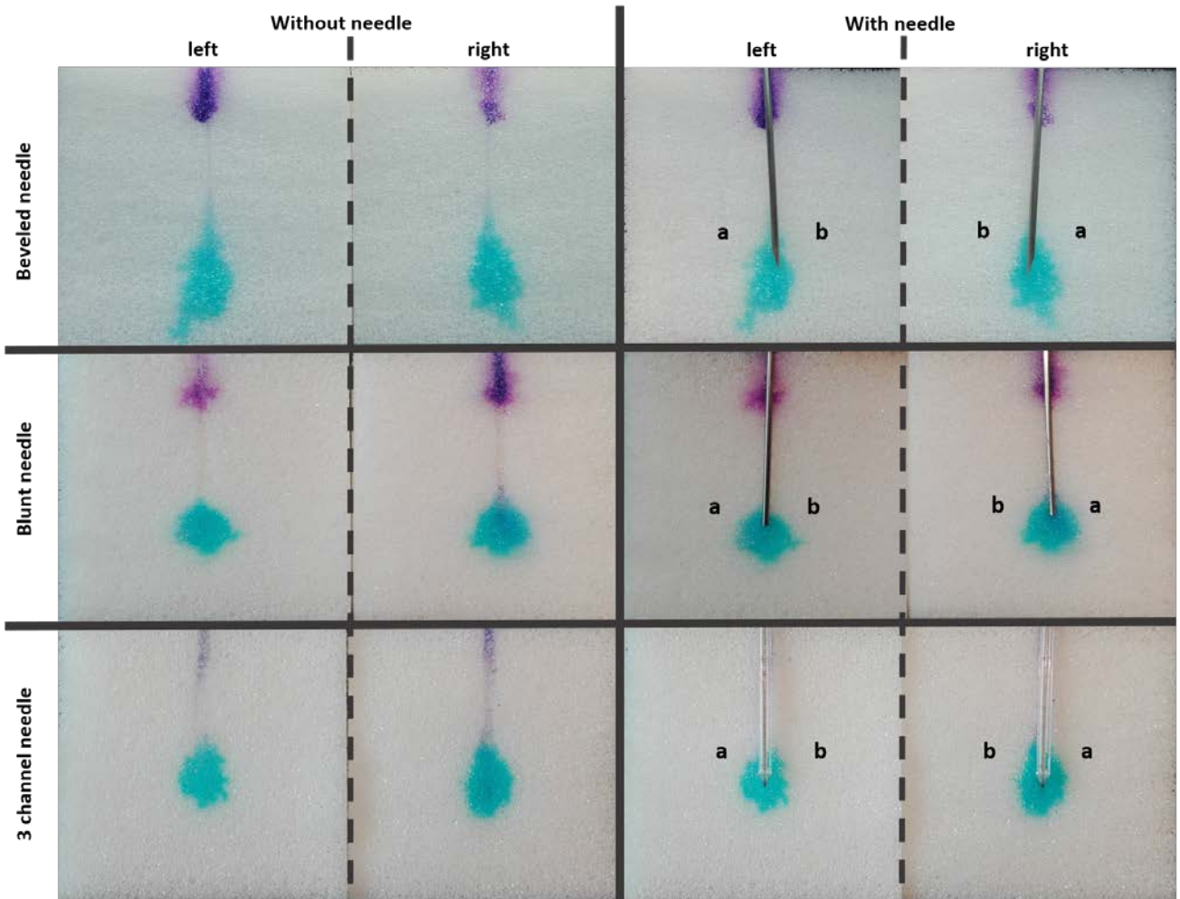
Figure 5: Experimental results. First row shows the results for bevelled needle, second row the results for the blunt needle and the last row the results for the 3-channel needle.
