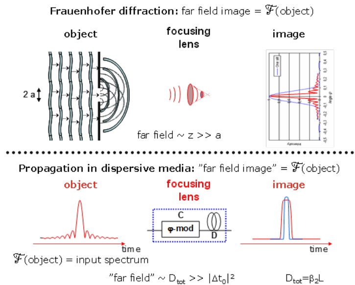
Figure 1 – Illustration of the parallel formalism for diffractive and dispersive Fourier transformation.
