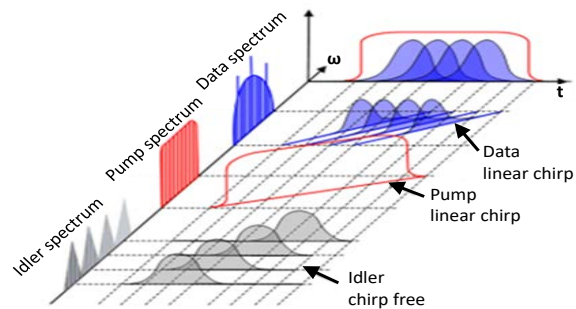
Figure 2 - Illustration of FWM used to apply phase modulation to an already chirped data signal. Chirp and phase modulation are matched to create a chirp free idler.
