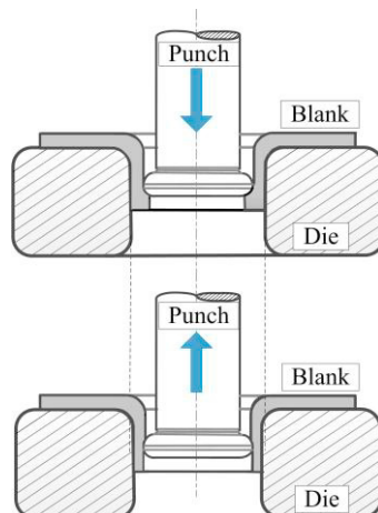
Fig. 1. Schematic of the ironing process during forward and backward strokes.
