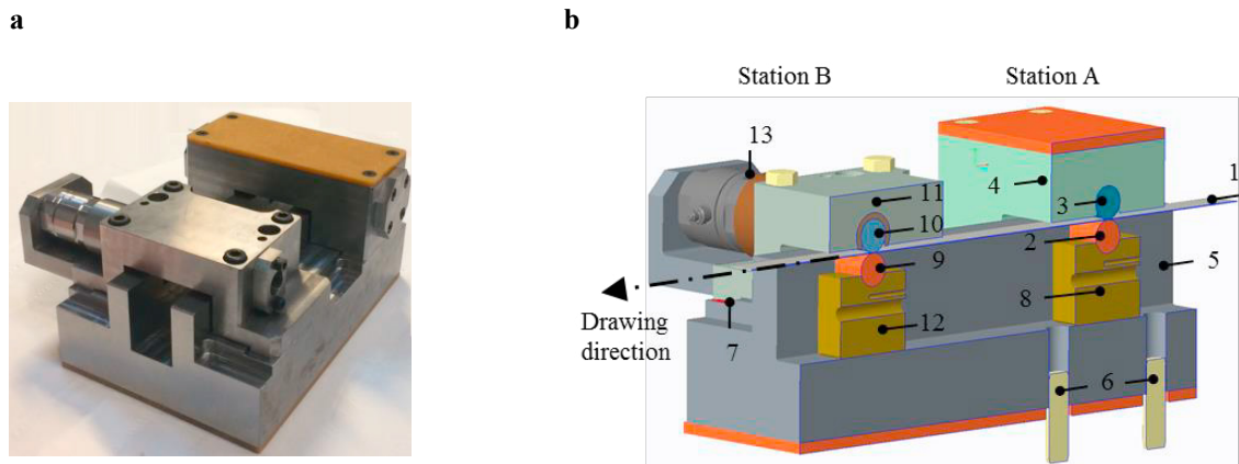
Fig. 2. (a) Photograph of the new SRT tool design and (b) schematic cross-sectional view of its main components.
