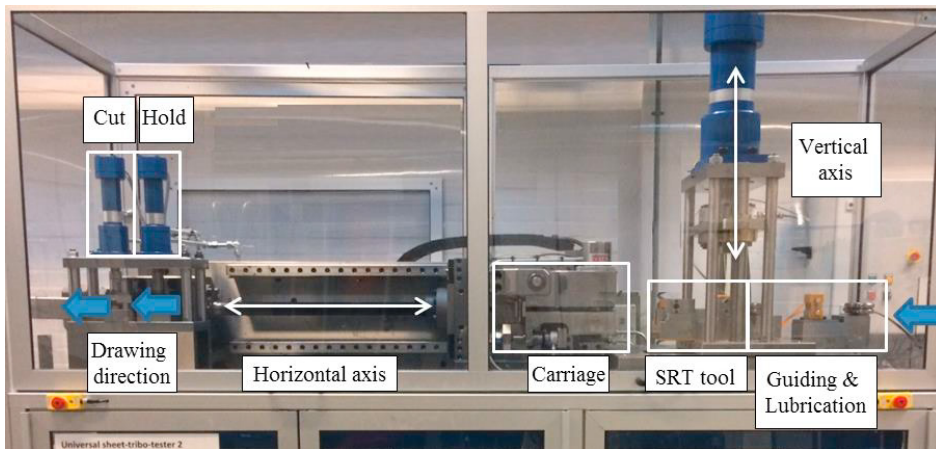
Fig. 3. The UST equipped with the new proposed SRT tool setup.
