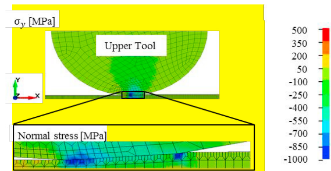
Fig. 4. Finite element distribution of \sigma_y for ‘Station A’ of the SRT tool setup with the detail of contact pressure.
