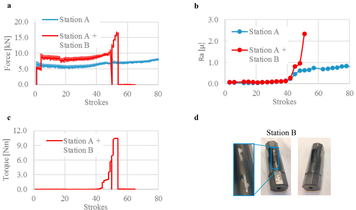
Fig. 5. Evolution of the (a) drawing force, (b) average strip surface roughness and (c) torque as function of the number of strokes, and (d) photographs showing pick-up formation on the tool surface.
