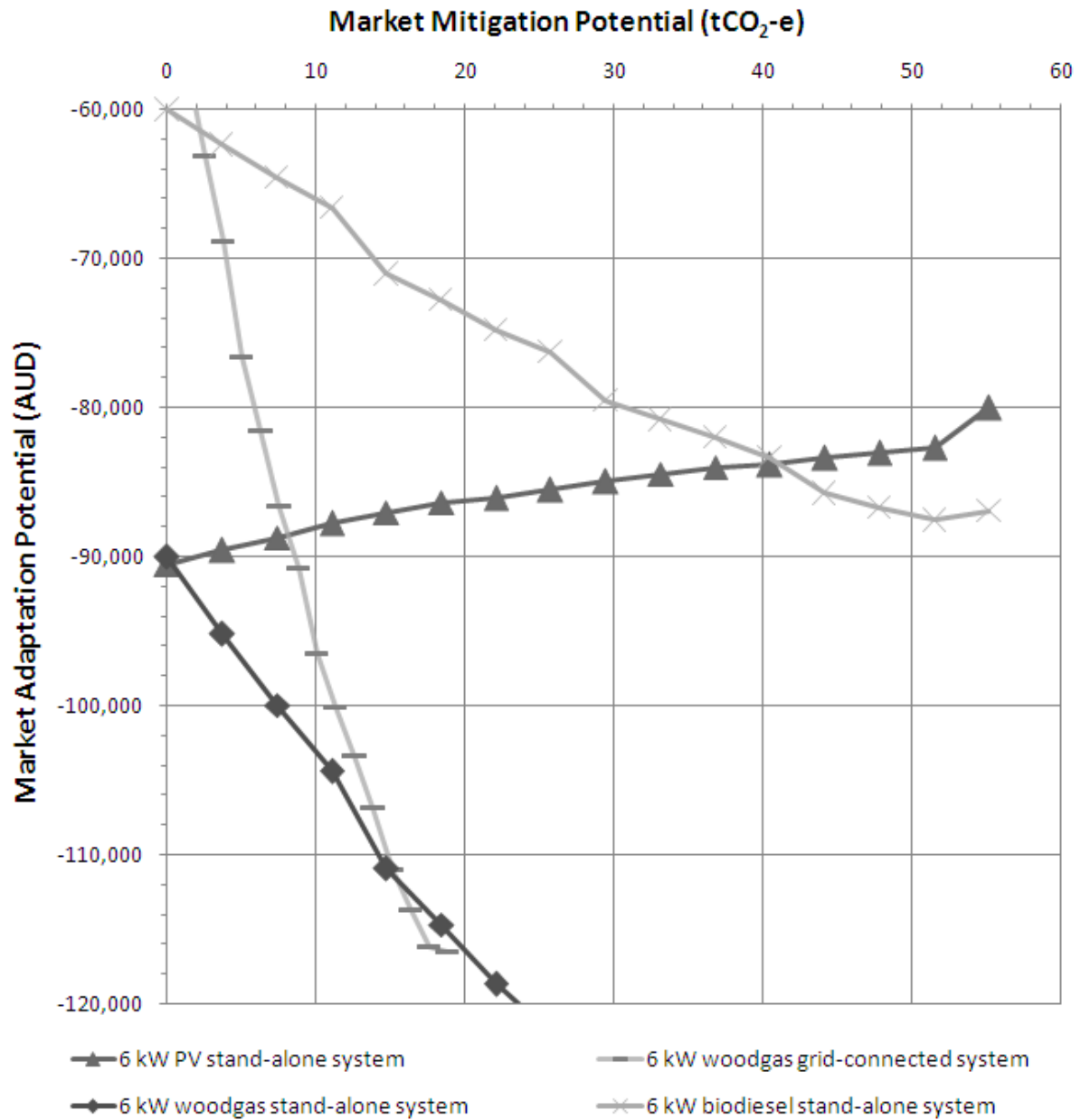
Fig.10. The total market adaptation potential (AUD) and market mitigation potential (tCO 2 -e), for the four 6 kW e system and scenario models at coordinates between zero and sixty tCO 2 -e, and AUD-60,000 and AUD-120,000.
