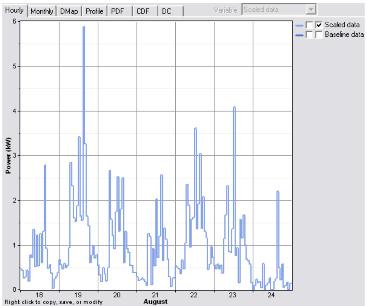
Fig. 5. Simulated 15 minute interval homestead electrical load profile.
