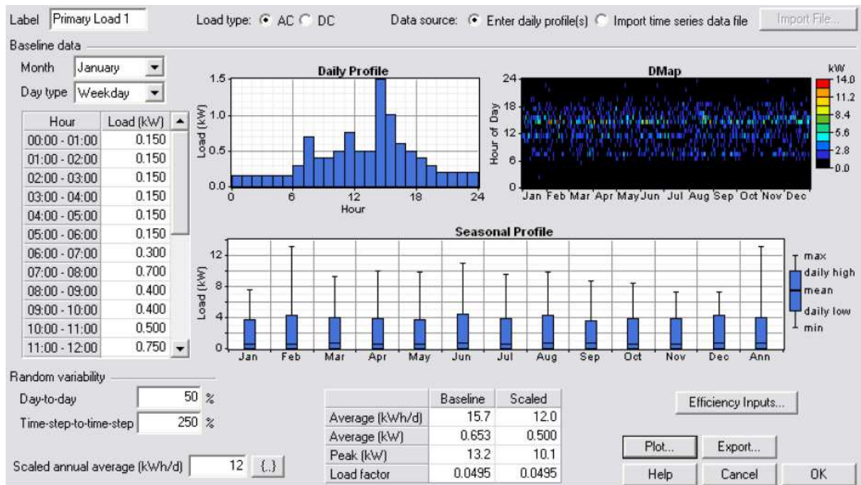
Fig. 6. Simulated intra-hourly, hourly, daily, and monthly electrical load profiles for the homestead.
