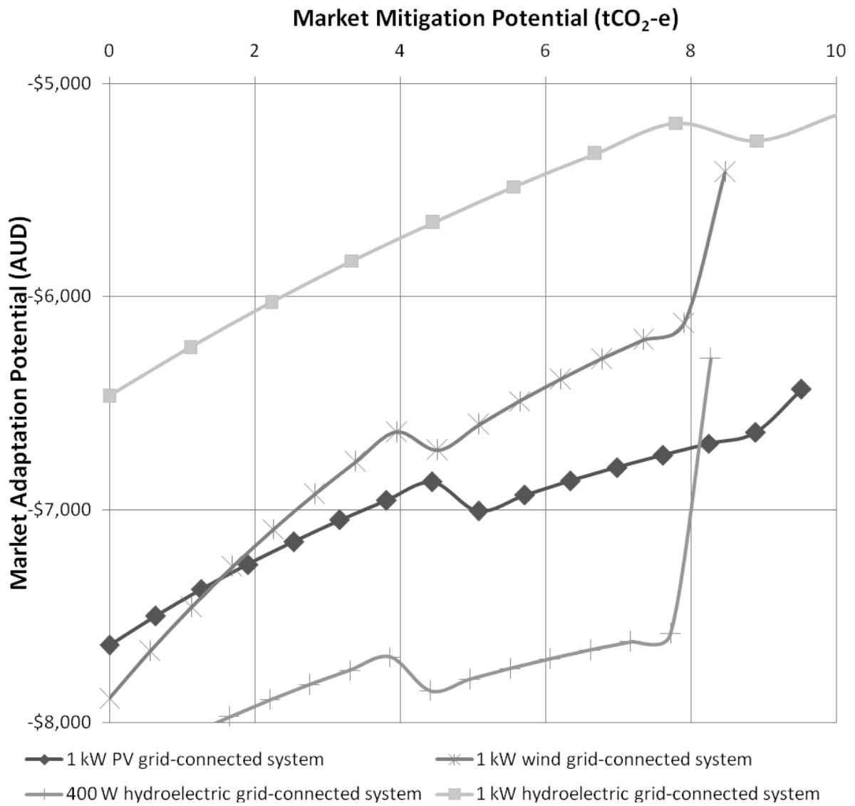
Fig. 9. The total market adaptation potential (AUD) and market mitigation potential (tCO 2 -e), for selected small-scale (≤1 kW) system models at coordinates between zero and ten tCO 2 -e, and AUD-5,000 and AUD-8,000.
