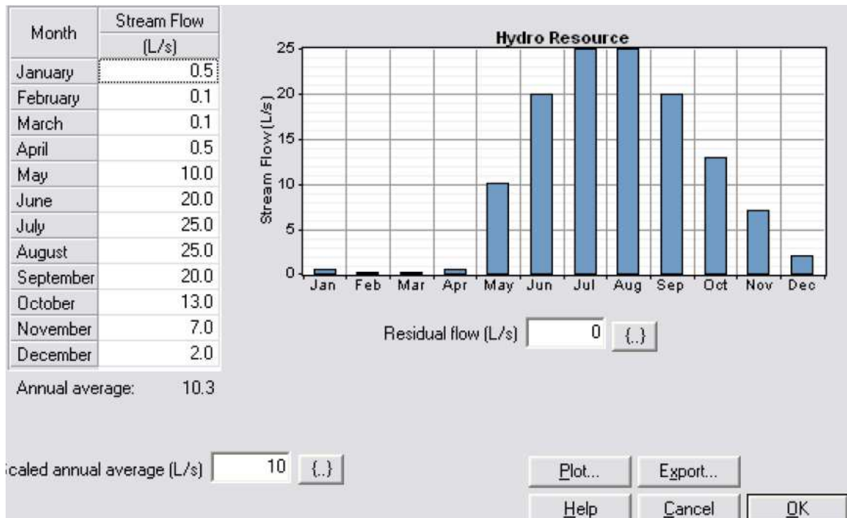
Fig. 4. Generated annual and monthly mean available river flow for hydro-electric simulations.
