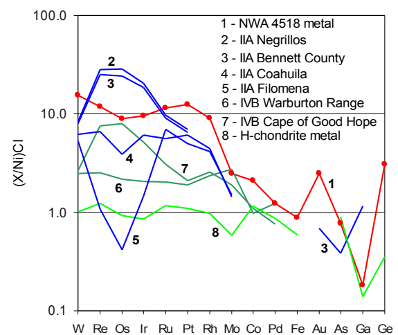
Fig. 2. Composition of the NWA 4518 metal in comparison with IIA [9-11], IVB [5] irons and H-chondrite metal [12] (normalized to Ni and CI).
