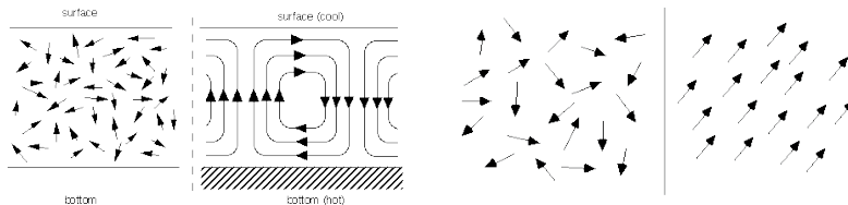
Figure: The left hand side picture display Bénard Rolls. The right hand side picture display the magnetisation phenomena.
