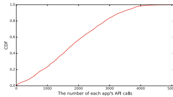
Fig. 9. CDF plot of the number of each app's API calls.
