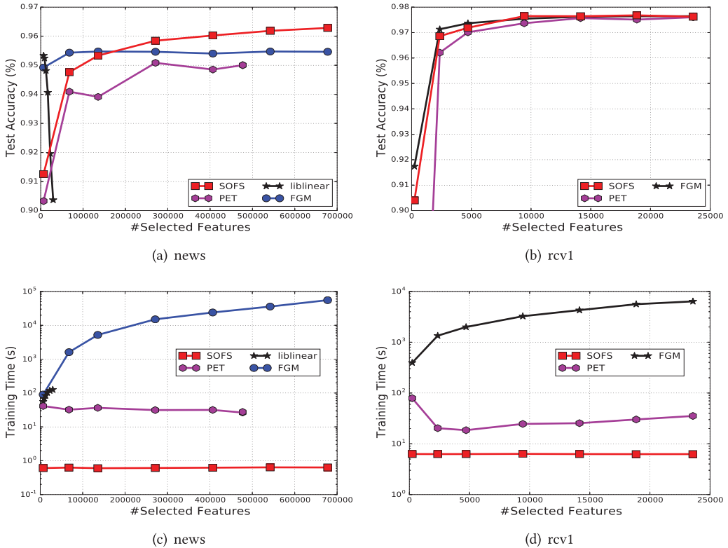
Fig. 6. Test accuracy and time cost versus number of selected features on the “news” and “rcv1” dataset.
