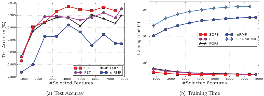
Fig. 5. Test accuracy and time cost versus number of selected features on the caltech dataset.
