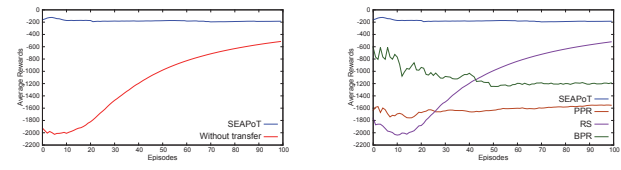
Figure 2: Performance of SEAPoT versus no transfer
