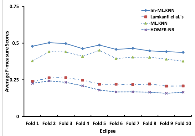
Fig. 10. Experiment Results of Im-ML.KNN, Lamkanfi et al.'s approach, ML.KNN, and HOMER-NB for Eclipse with different folds.
