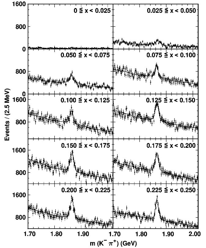
FIG. 12. The m(K^- \pi^+) distribution for B \rightarrow D^0 X candidates in ten x bins from 0 to 0.25. The histogram is the result of the fit.
