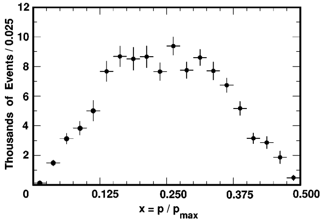
FIG. 16. The background-subtracted and efficiency-corrected yield of D^0 mesons from B \rightarrow D^0 X decay, as a function of scaled momentum ( p_{\max} = 4.950 \text{ GeV}/c ).
