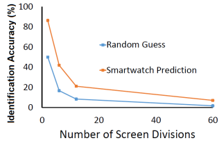
Fig. 5: Prediction accuracy vs. number of screen divisions
