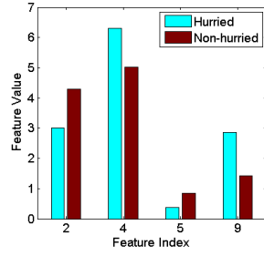
Fig. 4: Values of dominant features listed and indexed in Table IV respectively. All durations are in seconds
