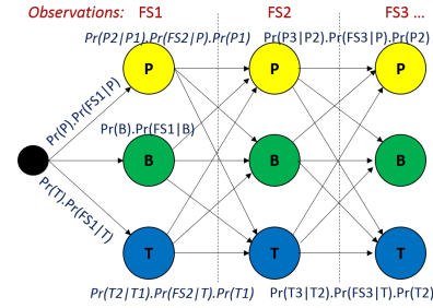
Fig. 7: Trellis diagram corresponding to the Viterbi decoding of hand action sequences.
