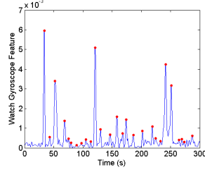
Fig. 6: Watch gyroscope feature peaks indicating potential hand activities. The red dots show the actual hand activities from ground truth.
