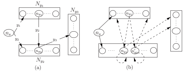
Figure 3: Part (a) shows an example of a HBC with three observations. Part (b) shows the warm-start strategy with dotted lines corresponding to variables to be optimized.
