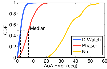
Figure 10: LoS AoA estimation with proposed calibration method.
