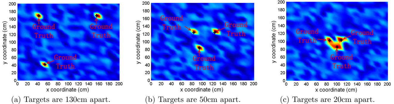
Figure 19: Performance of multi-target localization. (a)-(c) show the heatmaps of three snapshot localization results.
