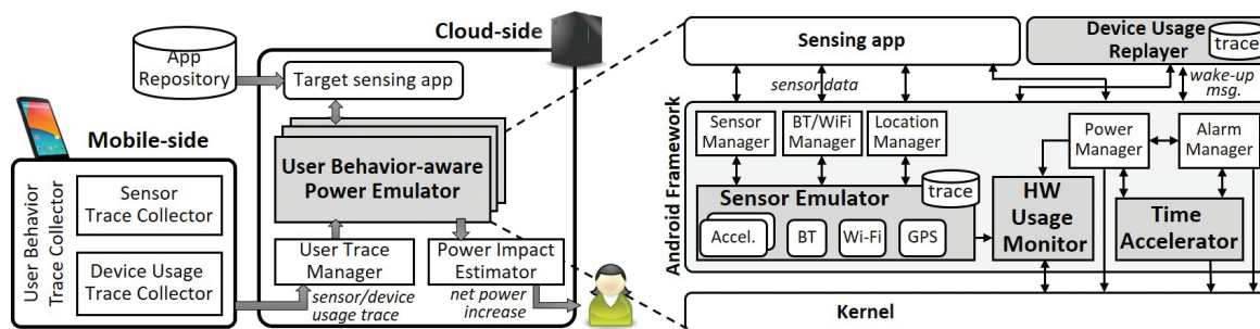
FIGURE 2. PowerForecaster architecture.
