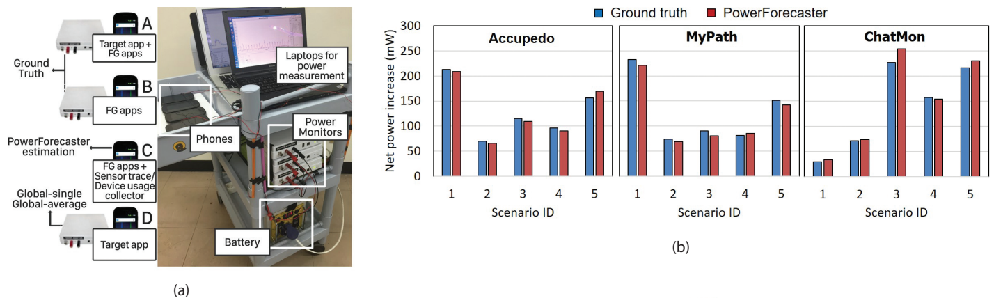
FIGURE 3. PowerForecaster evaluation: (a) setup (left), (b) estimation accuracy (upper right), and (c) latency (lower right).
