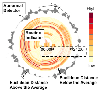
Fig. 4: Road Fingerprint View Design. Road fingerprint displays the routine pattern in the center, surrounded by temporally distributed historical attributes. A new visual component, "similarity lens", including a "routine indicator" and "abnormal detector" is presented. A routine indicator is bar chart like glyph structure and each bar represents a time period (hour or day). The height encodes the value. An abnormal detector is the outer glyph lying on the furthest ring. It has a routine line which indicates the average value. Each big sector on the cycle represents a day that has a related mapping part on the glyph.
