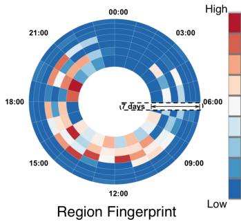
Fig. 3: The Region Fingerprint View Design. It uses a ring-map-based radial layout design to help explore historical statistical information. It shows the encoding scheme, which uses the typical heat map color, set represent density and the ring sectors around the fingerprint show the value of different time periods of the day.
