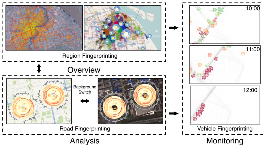
Fig. 2: The system’s work flow. The system uses preprocessed vehicle GPS data as input and has three major components: region fingerprint, road fingerprint, and vehicle fingerprint. The region fingerprint displays the whole spatial temporal distribution and uses the ring-map-based radial layout design to discover historical data. The road fingerprint can further analyze interesting locations selected from the region fingerprint. The vehicle fingerprint can help explore historical statistical information while monitoring the real-time situation.
