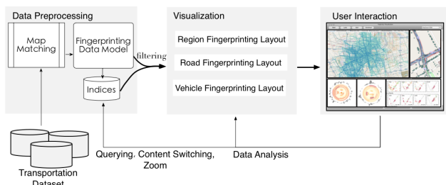
Fig. 1: The system architecture. The T-Watcher architecture consists of three primary components: (1) a data preprocessing module, (2) a visualization rendering module, and (3) a user interaction module.
