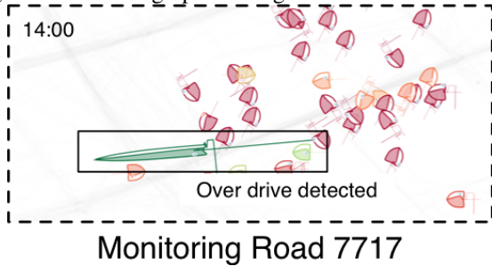
Fig. 10: Monitoring Result of Road 7717. It clearly detects an over drive situation.
