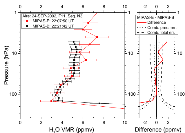
Fig. 1. Comparison of H 2 O profiles (left panel) measured by MIPAS-B (flight no. 11, sequence N3, black squared line) and MIPAS-E (orbit 2975, red squared line) on 24 September 2002 above southern France along with difference (right panel, red solid line), 1 \sigma combined precision (black dotted lines) and total errors (black dashed lines). Line styles are shown in the figure legend.
