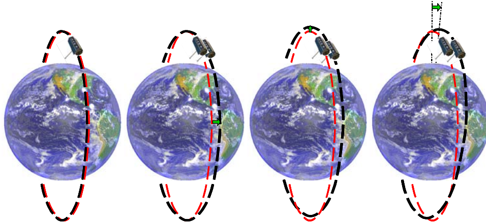
Figure 2. Formation building with relative eccentricity / inclination vector separation. From left to right: (1) identical orbits, (2) horizontal separation at equator crossings by small offset in the ascending node (green arrow indicates RAAN offset), (3) small eccentricity offset causes different heights of perigee / apogee and hence yields radial separation at poles. (4) Optional rotation of the argument of perigee to achieve larger baselines at high latitude regions.
