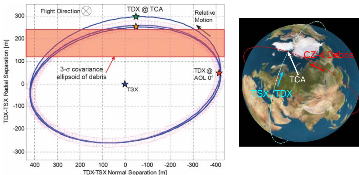
Figure 8. TDX-TSX / CZ-4 relative motion (left) and close approach geometry (right) at TCA (2011/03/25 15:08:11 UTC). Left: CZ-4 debris location is depicted as 3- \sigma covariance ellipsoid (red area). TDX position at TCA after avoidance maneuver execution is shown as green star. Without maneuvering TDX (orange star) would have been very close to the debris uncertainty ellipse. Because of the fact that TSX and debris planes were nearly perpendicular to each other (right), the debris along-track uncertainty directly maps into uncertainty in normal direction within TSX Hill frame (left). Therefore the debris uncertainty appears more like a band than an ellipse.
