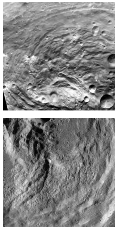
Figure 2: Arcuate ridge and scarp pattern across the floor of Rheasilvia (top – central complex is at bottom center) and within King crater on the Moon (bottom – central peak at upper left). King crater is 75 km wide.
