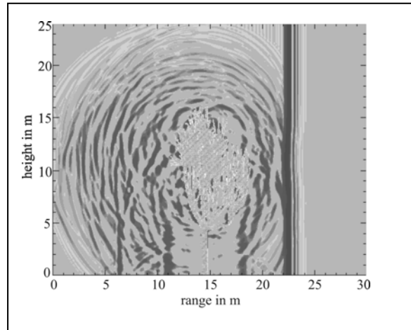
Figure 3: Snapshot of simulated sound pressure (vertical y-z cross-section through the centre of the domain) after the wave front has passed a row of idealized trees (type 1) from left to right
