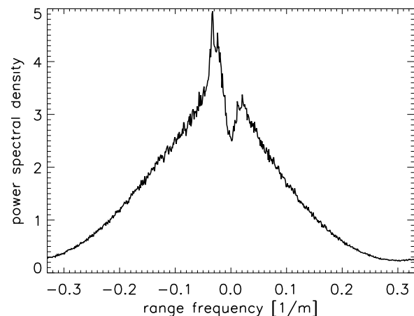
Fig. 2. The range spectrum of an interferogram (acquisition #1001508) over Brazilian rainforest. The spectrum is averaged over 2000 azimuth lines. The height of ambiguity is 25m.
