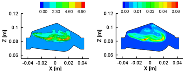
Figure 2: Root mean square of velocity (left) and mass fraction (right) at CA = 315°. Two-phase flow with variable spray boundary conditions.
