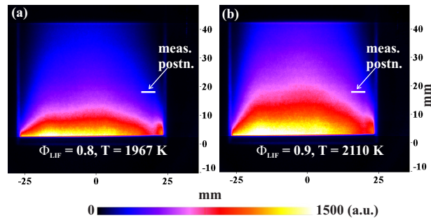
Fig. 3 2D OH LIF distribution of the investigated flames at 5 mm away from the edge of the matrix burner; also marked is the spatial position in the flame where the OH LIF spectral measurements were performed
