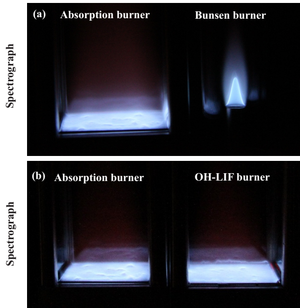
Fig. 1 Photographs showing the burner configurations that was employed in the current investigations. (a) OH* chemiluminescence signal trapping measurements (b) OH LIF signal trapping measurements
