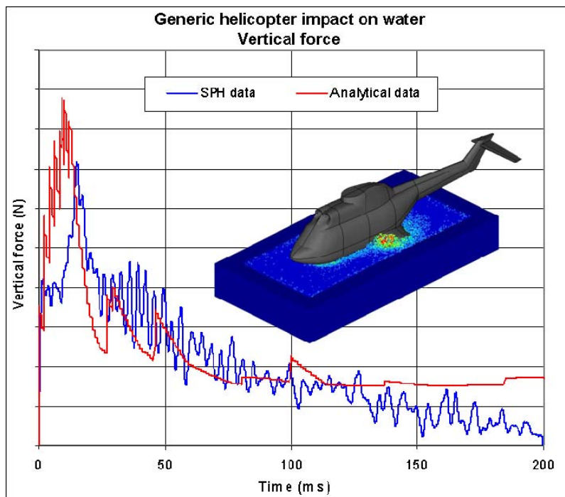
Figure 7 Comparison between SPH and analytical results - V_z=4 m/s / V_x=10 m/s / Pitch= 5^\circ
