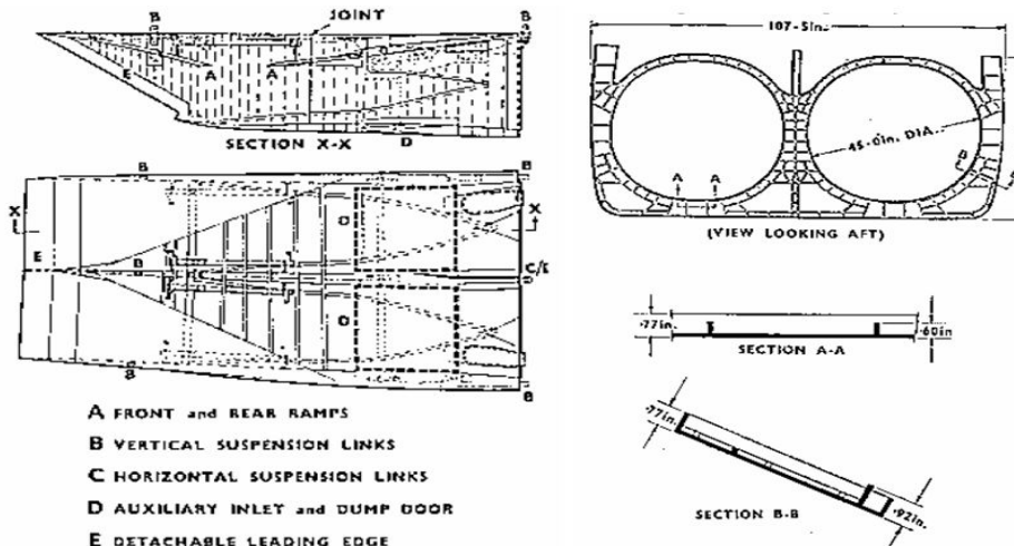
Figure 6: The concorde intake structure [35]
