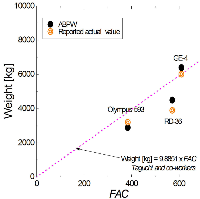
Figure 8: Estimation of turbojet engine weights
