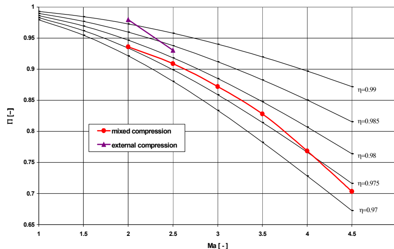
Figure 10: LAPCAT-M4-3R-V3 Air Intake geometry pressure recovery data
