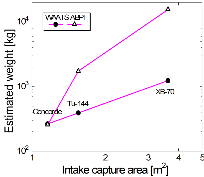
Figure 5: Estimated weight of several existing intakes (abpi and WAATS)
