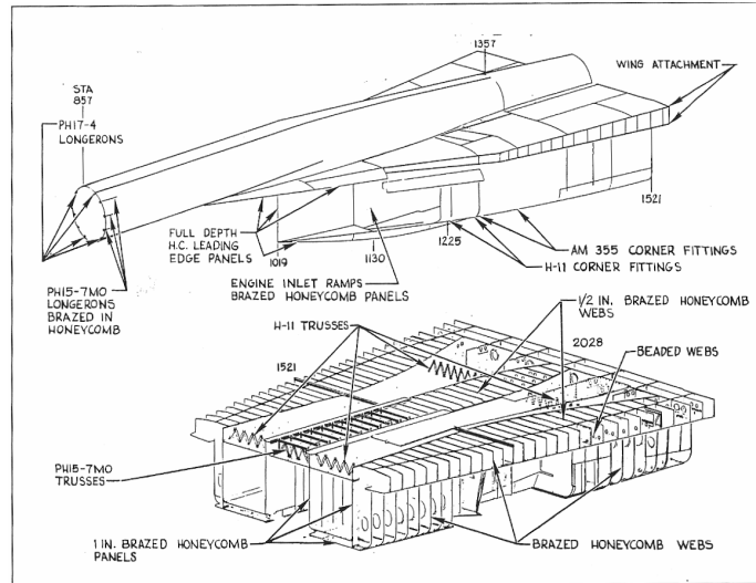
Figure 7: Materials and construction used in the upper and lower intermediate fuselage of XB-70 [36]
