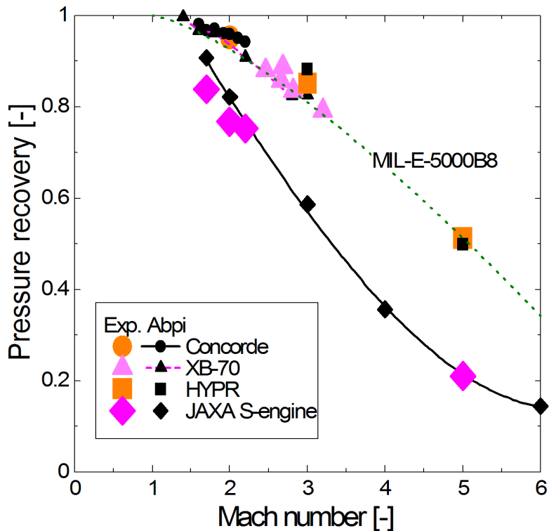
Figure 3: Pressure recovery data for existing intakes (dashed line shows MIL-E-5000B8).
