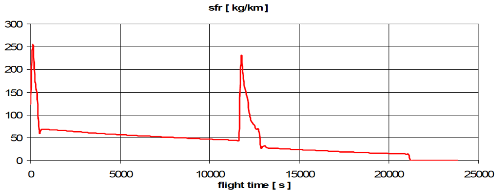
Figure 2: LAPCAT-M4 fuel consumption per range as a function of flight time [3]
