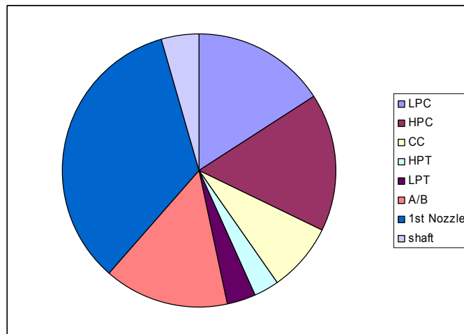
Figure 9: Weight distribution of major components by abpw calculation on Olympus 593
