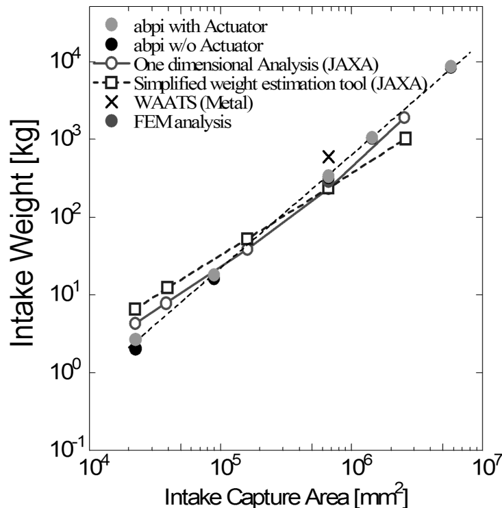
Figure 4: Validation of weight estimation tool by JAXA S-engine intake configuration
