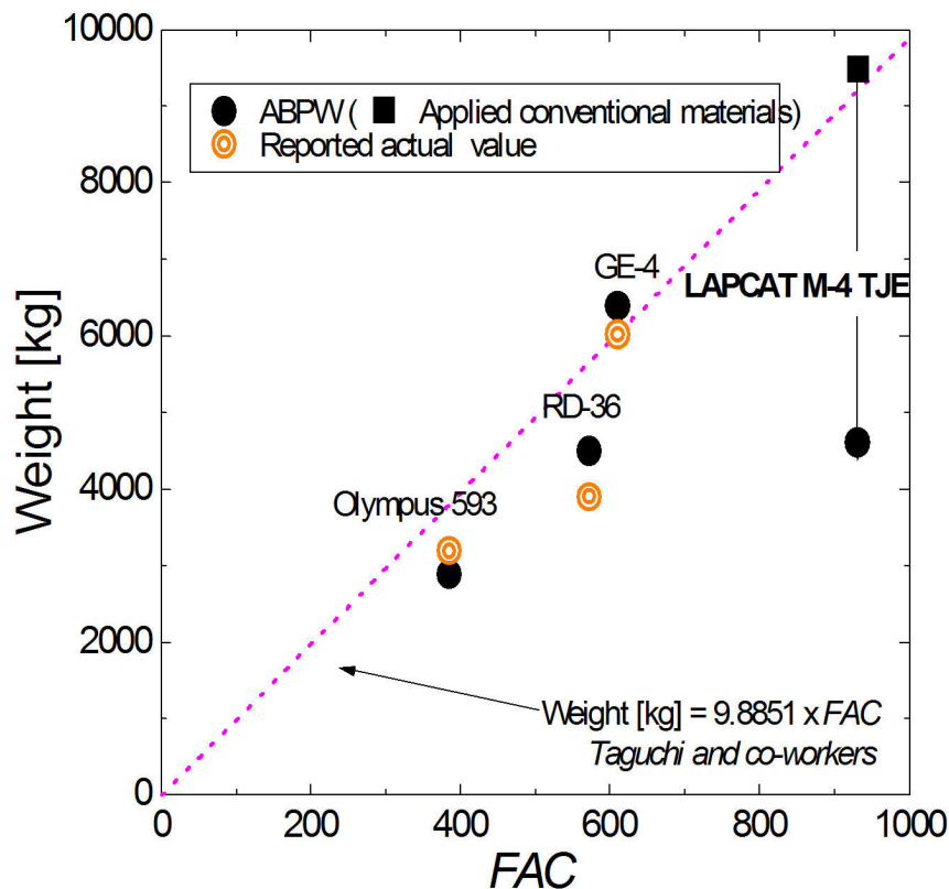
Figure 12: Engine weight estimation of LAPCAT TJE-6 and some existing turbojet engines
