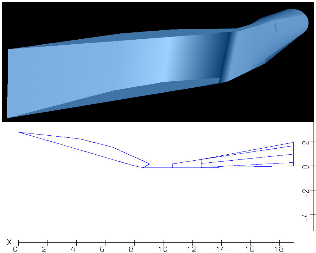
Figure 11: LAPCAT-M4-3R-V3 Air Intake geometry in wire-frame and shaded modes
