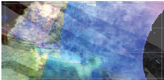
Figure 2: Western Xanadu as imaged by VIMS (RGB-Ratio-composit with R: 1.59/1.27 μm G: 2.03/1.27 μm B: 1.27/1.08 μm superimposed on Radar-SAR). Fluvial valleys are highlighted in light blue.
