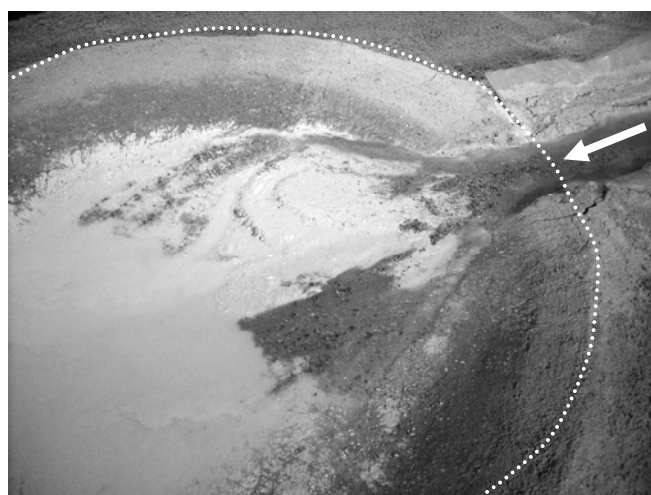
Figure 7. Thin layer of fine sediment draped over the deltaic deposit in the crater lake basin. Note the distinct elongate nature of the individual lobes, brought on by the increase in channel cohesion. Flow from right to left, with low discharge, and 20 % volumetric percentage of silica flour mixed with river sand.
