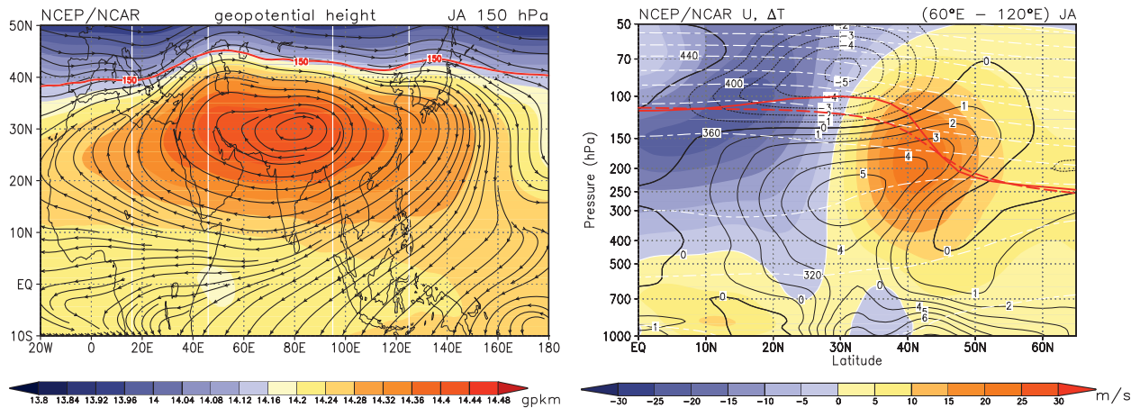
FIG. 2. (left) As in Fig. 1 but for the NCEP–NCAR reanalysis. The vertical white lines mark the sections used in Fig. 3. (right) Latitude–height sections between 1000 and 50 hPa from the equator to 65°N for the July/August long-term mean (20 yr) zonal velocity averaged between 60° and 120°E; shading interval 5 m s -1 . Displayed as contours in black are the temperature anomalies of the respective latitude section relative to the zonal average. The white dashed contours indicate the isentropic surfaces (contour interval 20 K). Displayed in red is the lapse rate tropopause: zonal mean (dashed) averaged between 60° and 120°E (solid). Data are from the NCEP–NCAR reanalysis.
