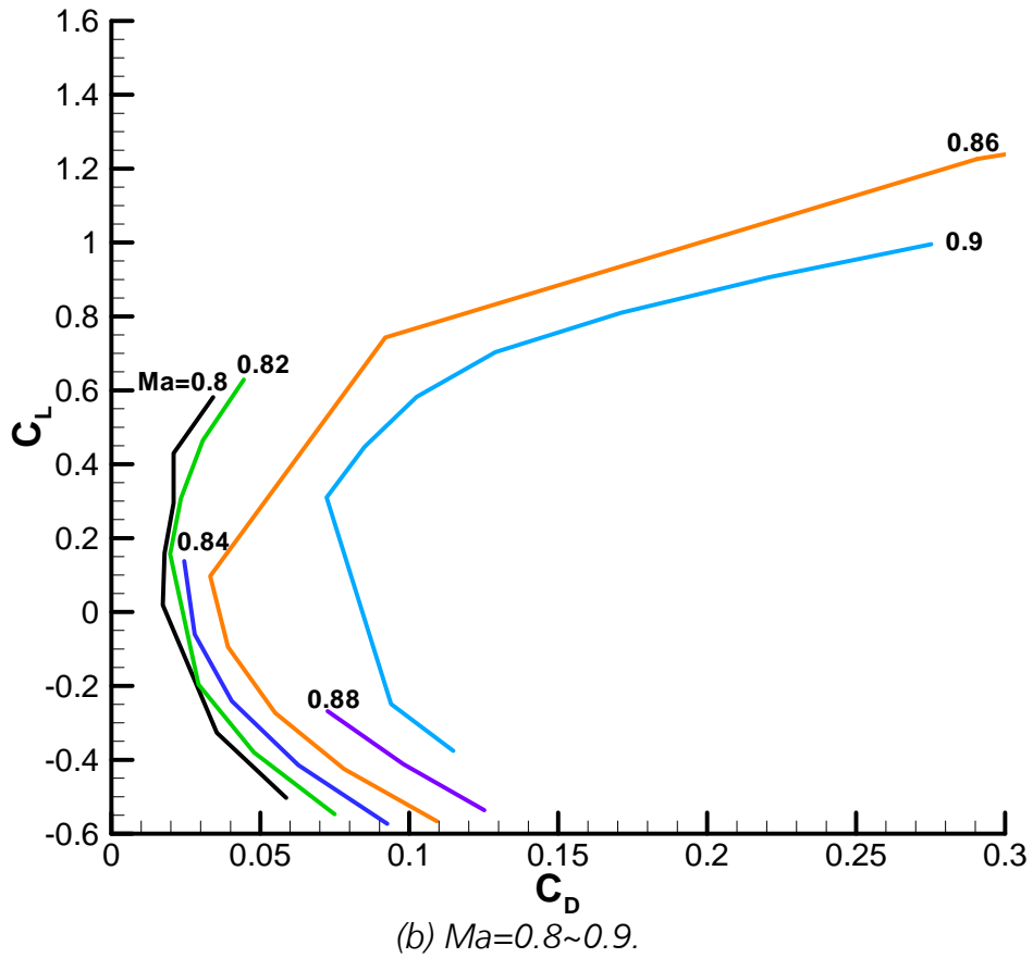
Fig. 15 Lift coefficient v.s. drag coefficient at different Mach numbers.
