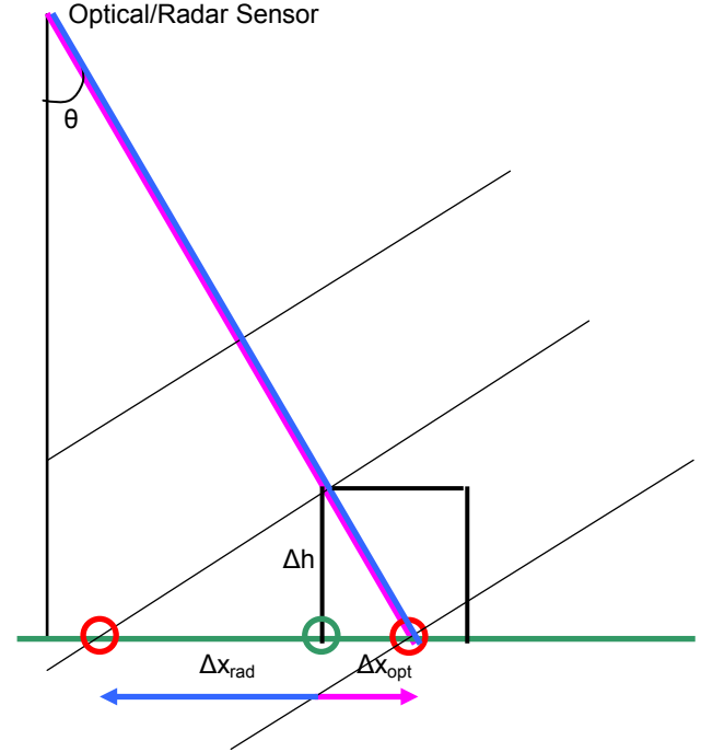
Figure 2. Ground displacement \Delta x for a 3D object of \Delta h height for an optical and radar sensor orthoimage. Look directions: pink line for optical sensor, blue line – radar sensor. The green horizontal line stands for a flat DEM, which doesn't include height information of objects. The green circle stands for a true ground position of a 3D point, whereas the red circle – a displaced position. Thin black line perpendicular to blue line shows approximately the radar wave propagation. Flight track is into plane.
